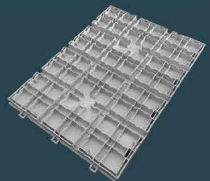
UNDERSIDE Durable Cross-Ribs
